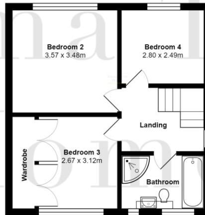
First Floor Area: 44.0 m 2
